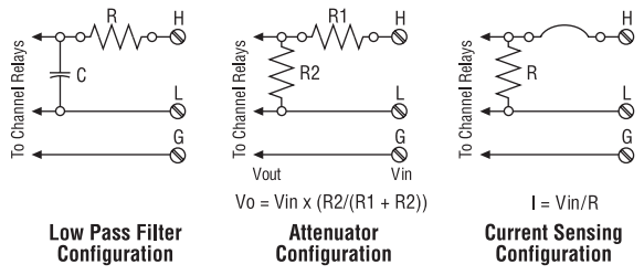
Signal Conditioning Components/Current Shunt
