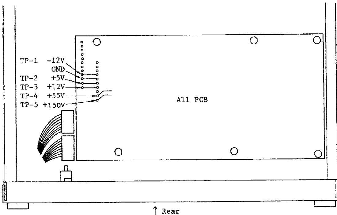
Figure 7-2 (Bottom view)
