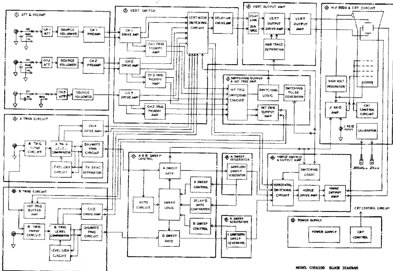
MODEL C066100 BLOCK DIAGRAM
