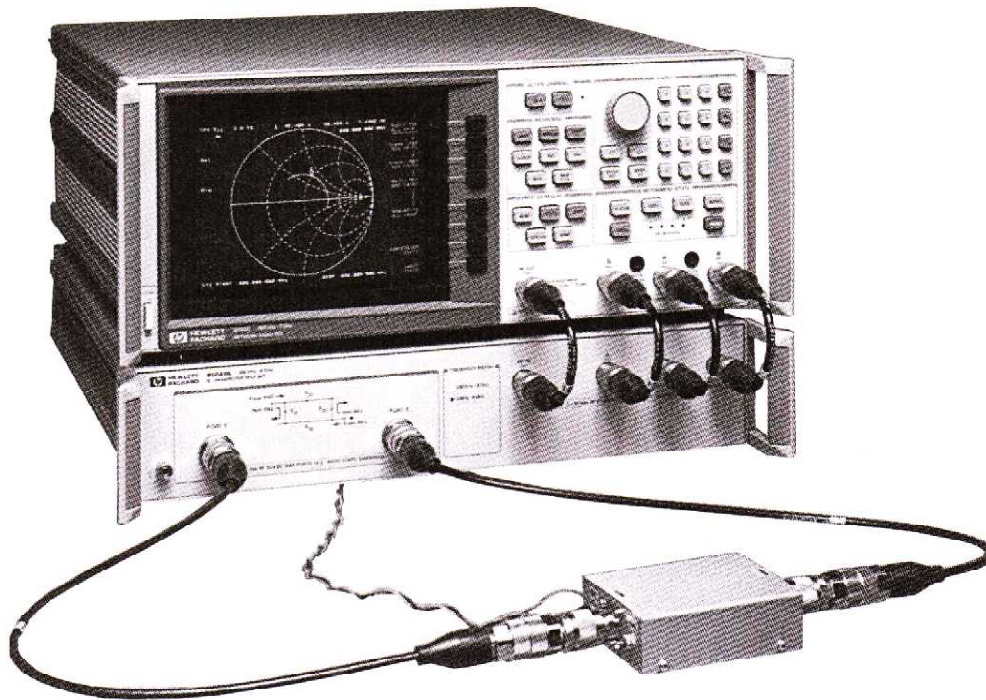
HP 8753C with HP 85047A
